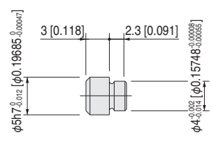
Locating pin: -P (P-MGA2)
