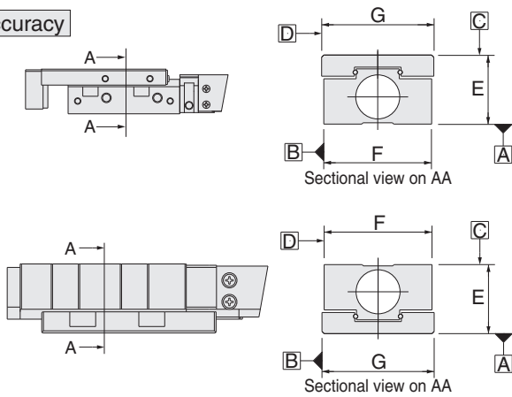
Mounting parallelism(face C relative to face A, face D relative to face B) mm [in.]
